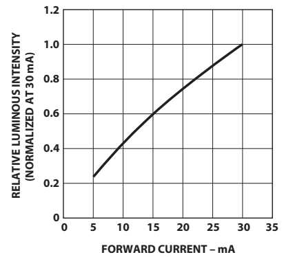
Figure 4. Relative intensity vs. forward current (InGaP)
